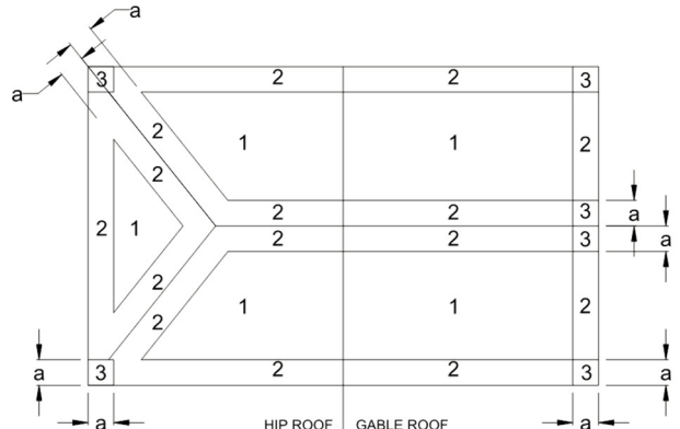
ROOF ZONES FOR GENERIC BUILDING
